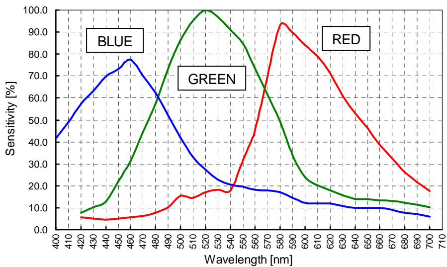
Spectral Sensitivity Specification for CSC12M25CMP19
