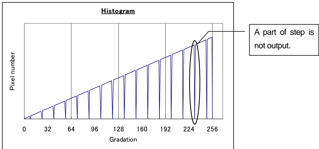
Fig 8.7. Example of outputting step of this camera(8bit output)
