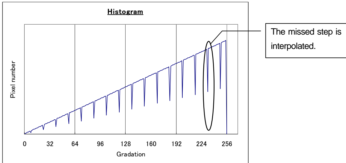
Fig 8.7.2. Example of step interpolation function (8bit output)
