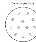
Picture Rear-camera connector (Rear-view)
