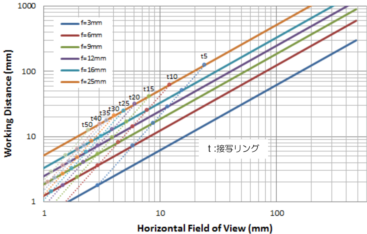
Working Distance vs Field of View of SPS
